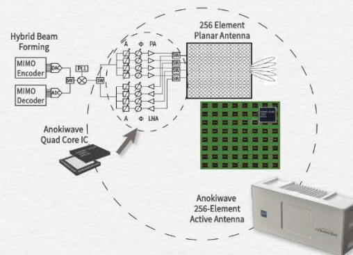
5G Antenna Array formation using AWMF-0108 and AWA-0134
